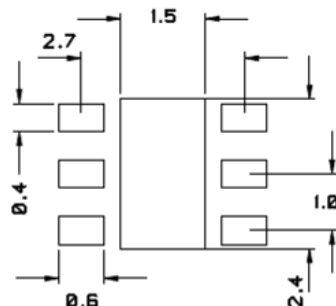
Recommended footprint for HTU21D sensors. Values in mm.
