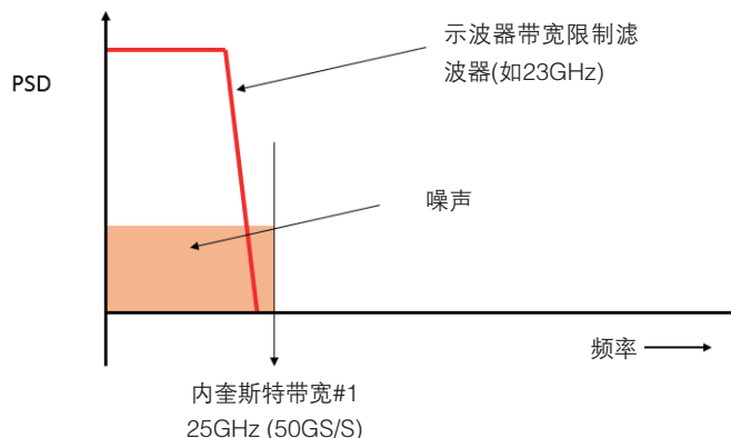
图2. 随机噪声power spectral density (PSD), relative to frequency.
